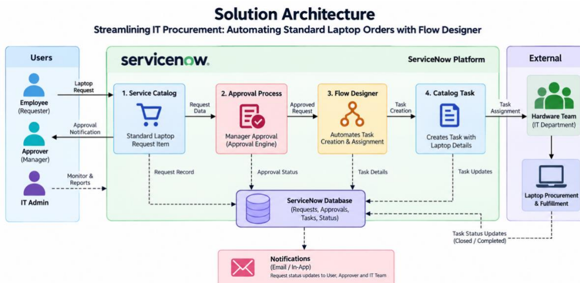
Figure 1: Solution architecture and data flow of the Standard Laptop Procurement automation using ServiceNow Flow Designer
